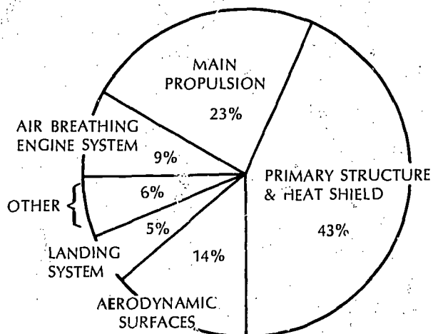
Fig. 4 TYPICAL DISTRIBUTION OF ORBITER DRY WEIGHT
